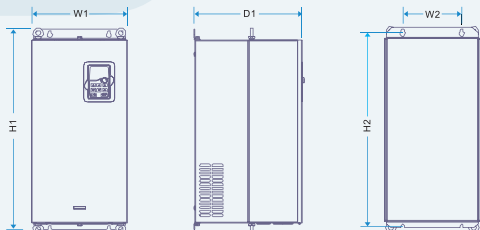
18.5-55kW Installation
